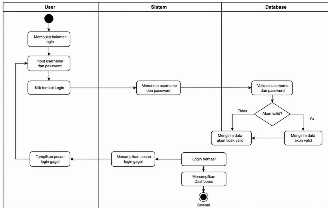
Gambar 3.3 Activity Diagram Login
