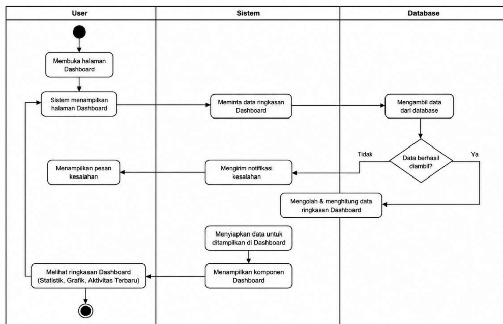
Gambar 3.4 Activity Diagram Dashboard
