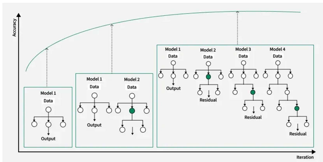
Gambar 2. 1 Metode Light Gradient Boosting Machine
